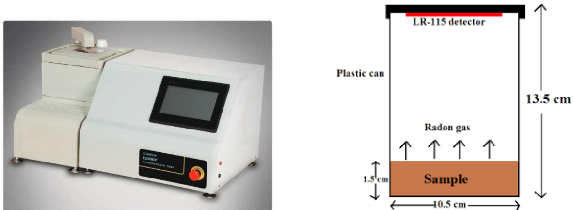
Fig. 2.1: Assembly for the measurement of radon exhalation rate using ‘ClosedCan Technique’ and Etchingbath
